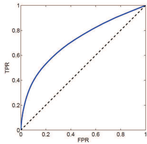
Figure A-1: ROC curve
