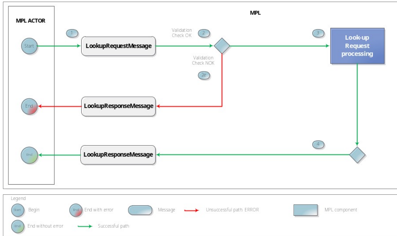
Figure 5 – Look-Up process
